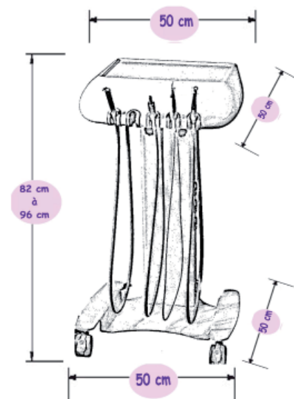
Dim Cart ref 1-380
