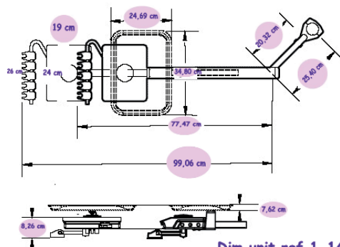
Dim unit ref 1-140
