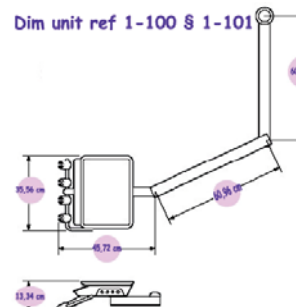
Dim unit ref 1-100 § 1-101
